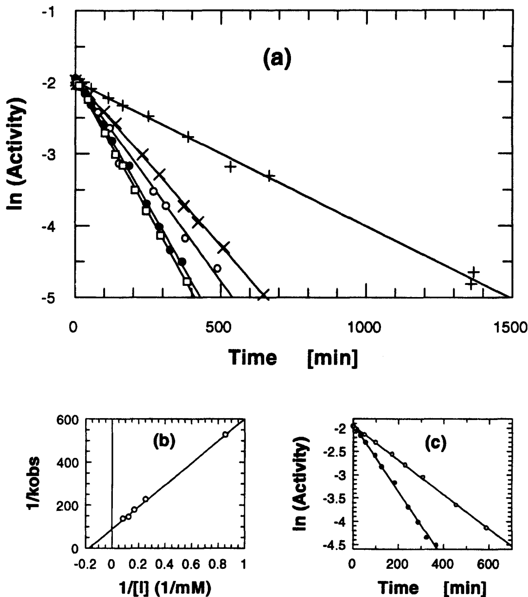
Figure 3. Determination of kinetic parameters for the inactivation of pABG5 by nitroglucal. (a) Time-dependent decrease in Abg activity with increasing concentrations of nitroglucal. Inactivation reactions were performed at 37 °C in 50 mM sodium phosphate buffer (pH 6.8.) with a fixed concentration of Abg and 0.1% BSA. Residual activity assays were performed as described in the text. The concentrations of nitroglucal in the inactivation reactions were 1.2 (+), 3.9 (x), 5.9 (o), 7.8 (●), and 11.7 (□) mM, and the values of k_{\text{obs}} were 0.0019, 0.0044, 0.0056, 0.0069, and 0.0073 \text{min}^{-1} , respectively. (b) A double-reciprocal plot of the k_{\text{obs}} values from (a). (c) Protection against nitroglucal inactivation by glucosyl benzene. Reactions were carried out with 7.8 mM nitroglucal and 0 (●) or 9.9 (○) mM glucosyl benzene: values of k_{\text{obs}} obtained were 0.0069 or 0.0036 \text{min}^{-1} , respectively.
