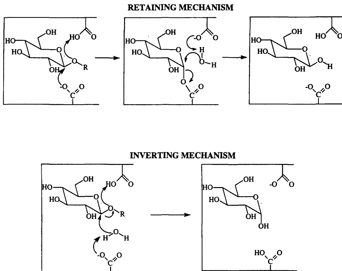
Figure 1. Mechanisms of inverting and retaining glycosidases.
